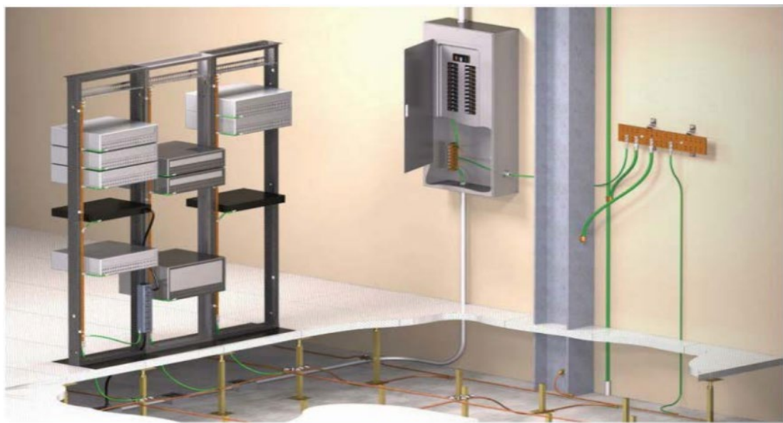
Figure 4: Grounding and Bonding in IT Equipment Room (from BICSI)
